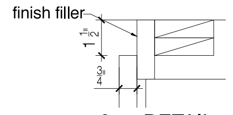
9. DETAIL
